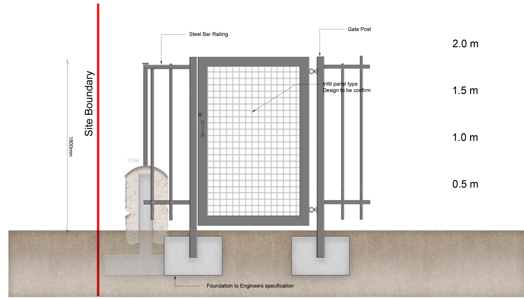
1 Landscape Elevation- Proposed controlled gate during the nighttime scale 1:20@A0
