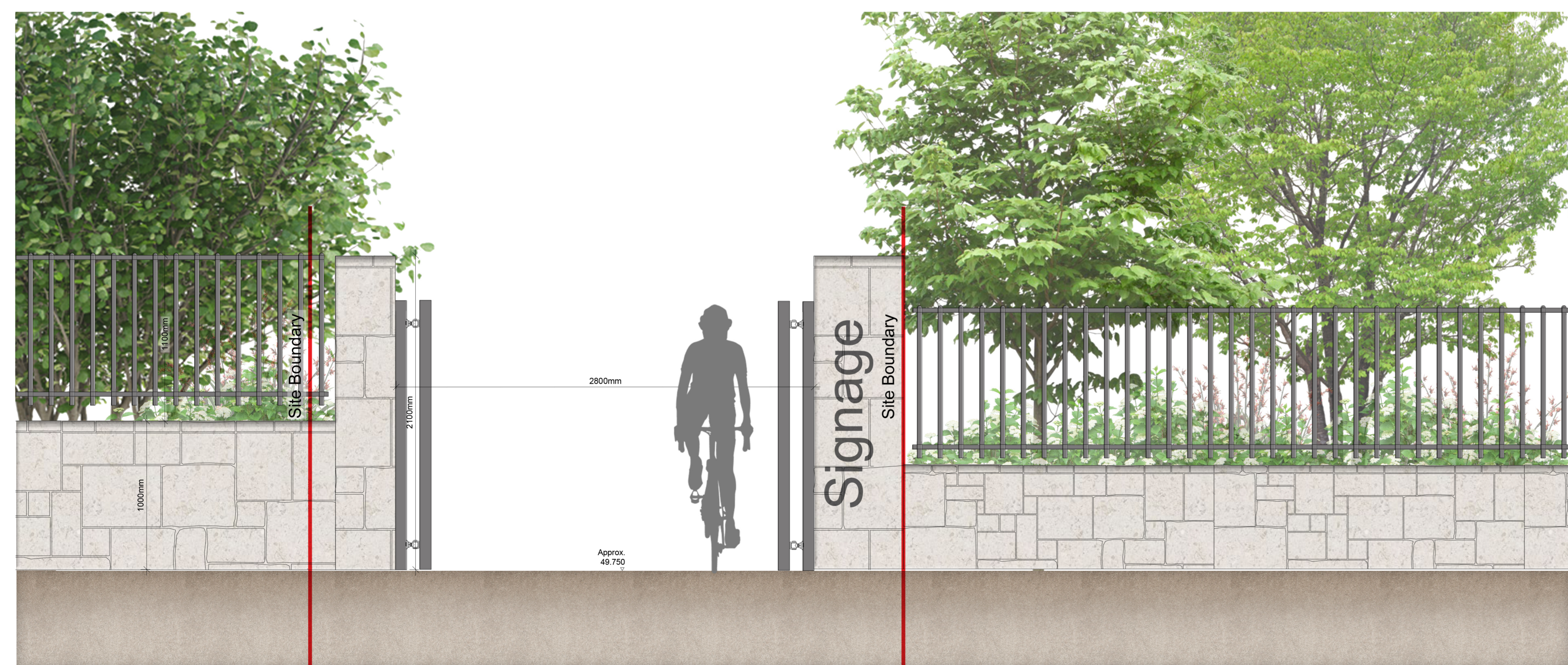
3 Landscape Elevation- Proposed access from N11 scale 1:20@A1
