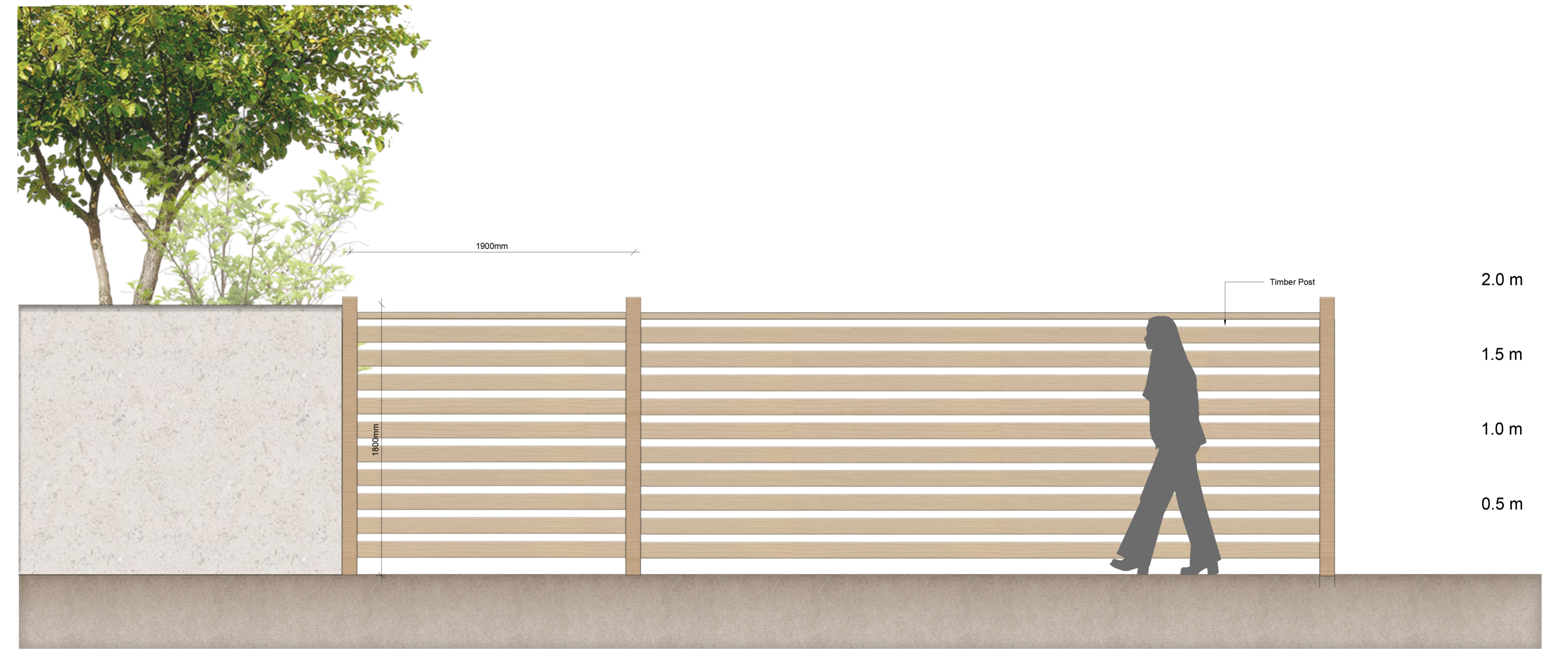
4 Landscape Elevation- Proposed rendered wall infill with timber fence allowance for future connectivity at Willow Grove scale 1:20@A0
